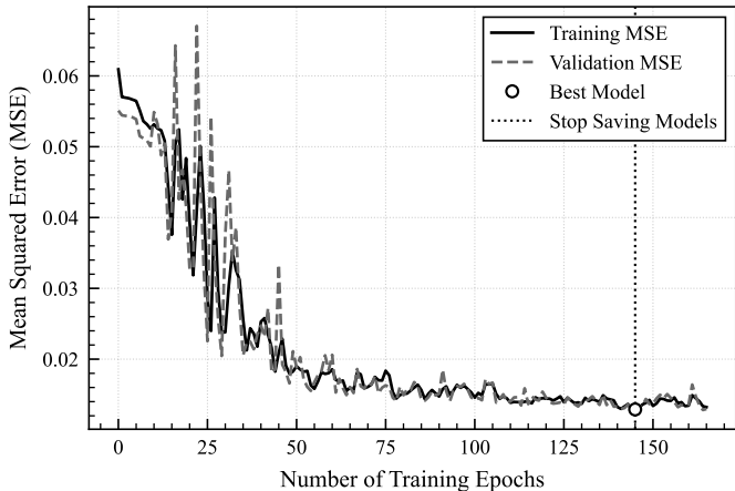
Learning Curve of MHSA-GRU Model for SolarPlant-1 (Gyeongju)
